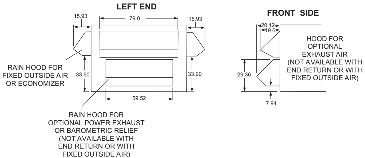
FIGURE 40 - CLEARANCES - HOOD/ECONOMIZER & MOTOR DRIVE - FRONT & END
