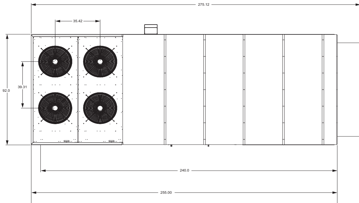
FIGURE 35 - 30 AND 40 TON MILLENNIUM OVERHEAD VIEW
