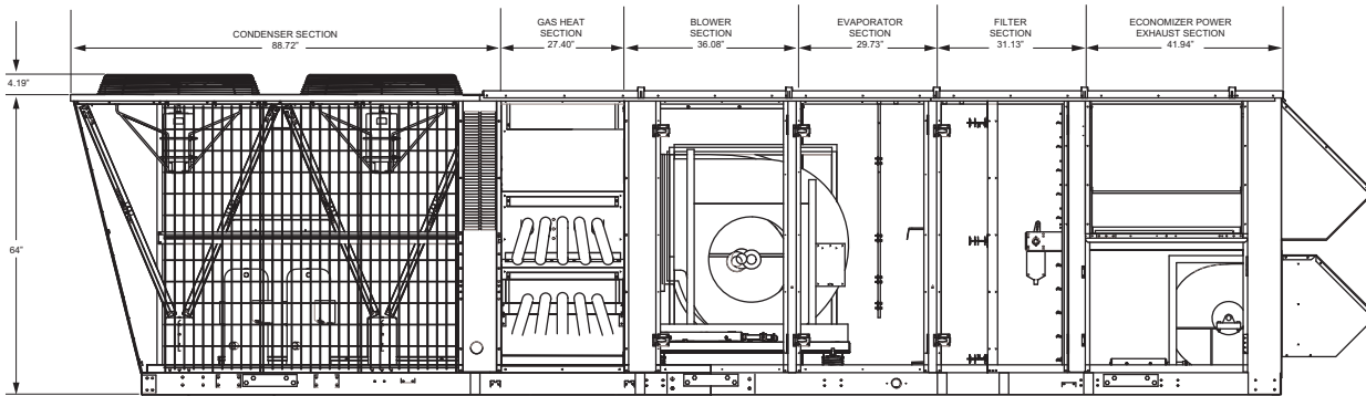
FIGURE 37 - 30 AND 40 TON MILLENNIUM MAJOR COMPONENT LAYOUT
