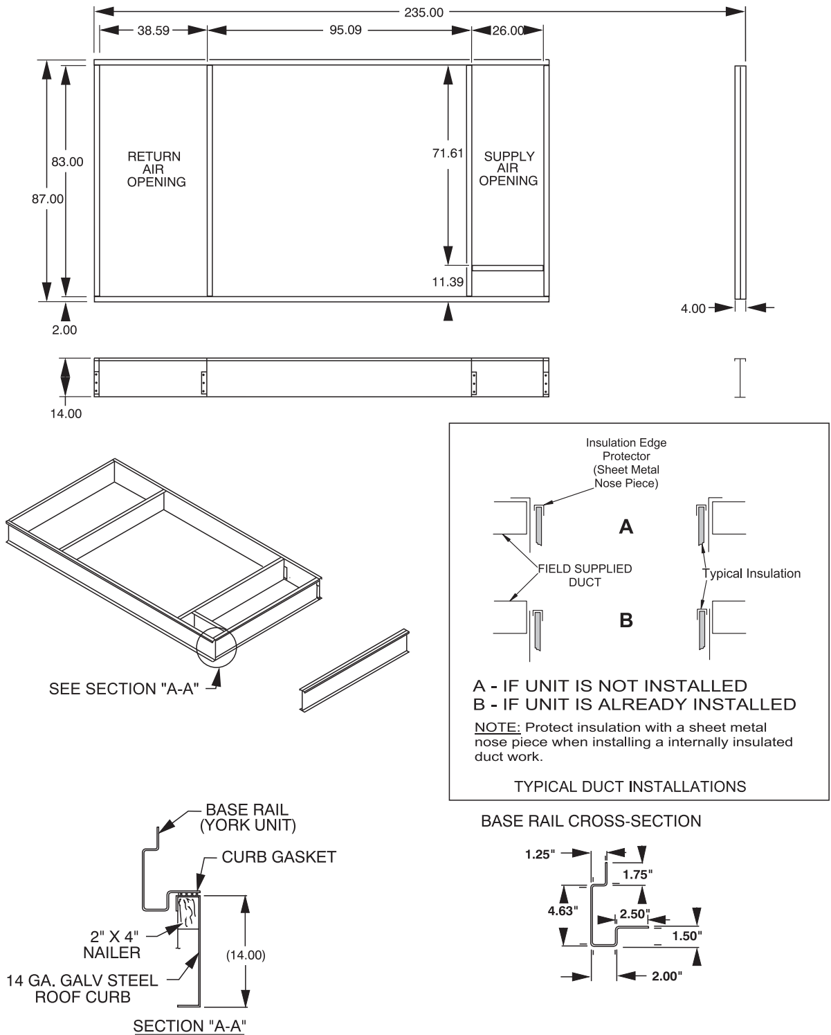
FIGURE 41 - PARTIAL ROOF CURB MODEL 1RC0455P
