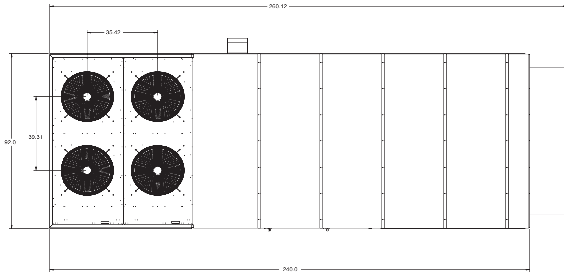
FIGURE 34 - 25 TON MILLENNIUM OVERHEAD VIEW
