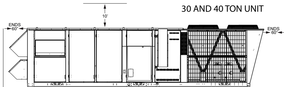
FIGURE 39 - CLEARANCES - HOOD/ECONOMIZER & MOTOR DRIVE - SIDE
