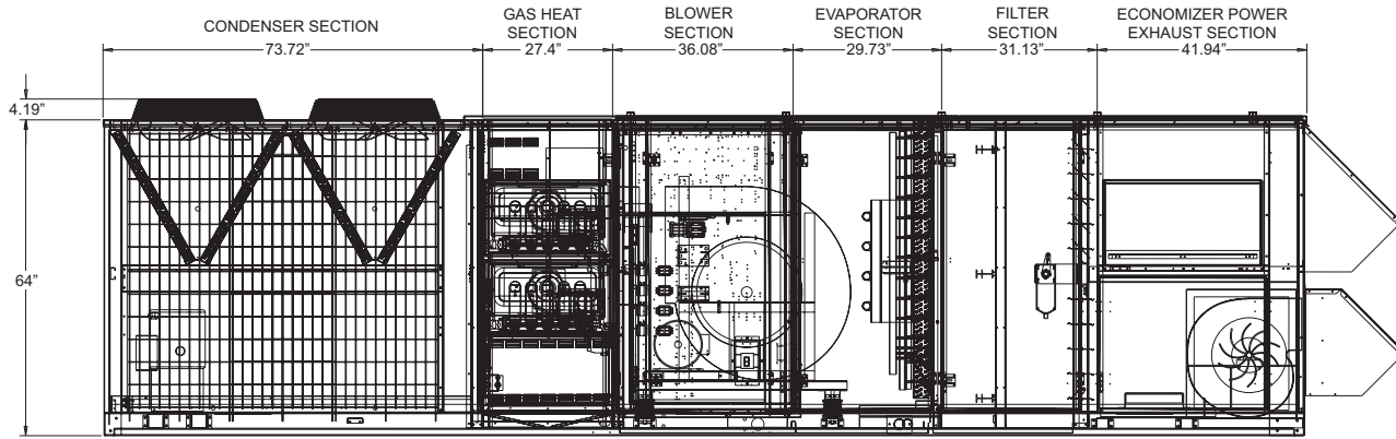
FIGURE 36 - 25 TON MILLENNIUM MAJOR COMPONENT LAYOUT
