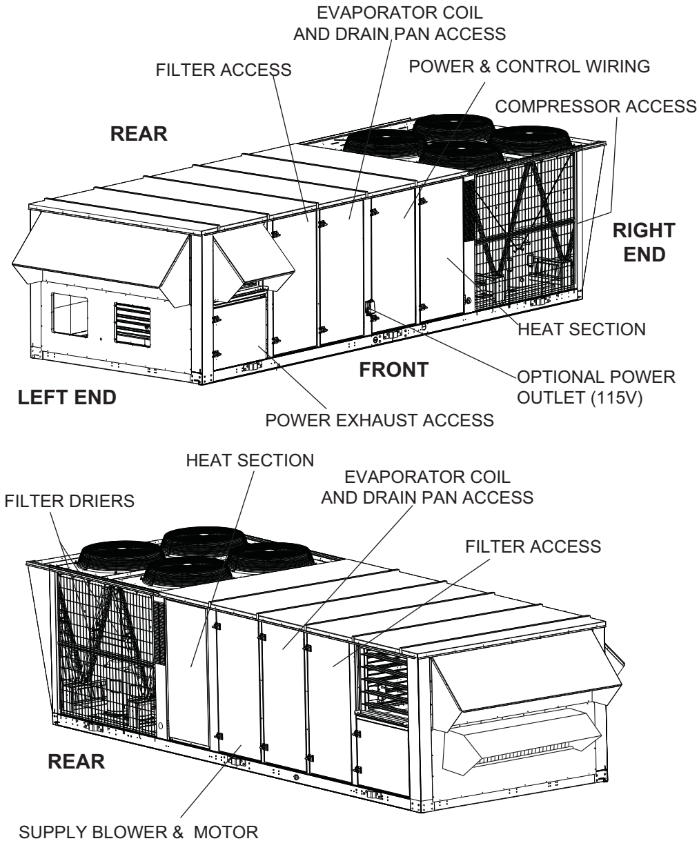
FIGURE 29 - COMPONENT LOCATION
